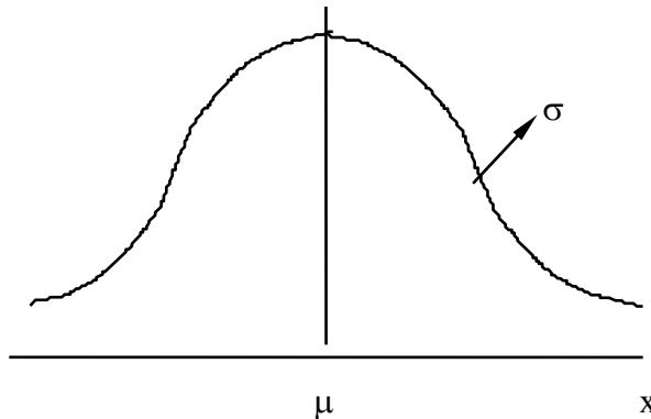
Gambar1. Kurva Distribusi Normal
